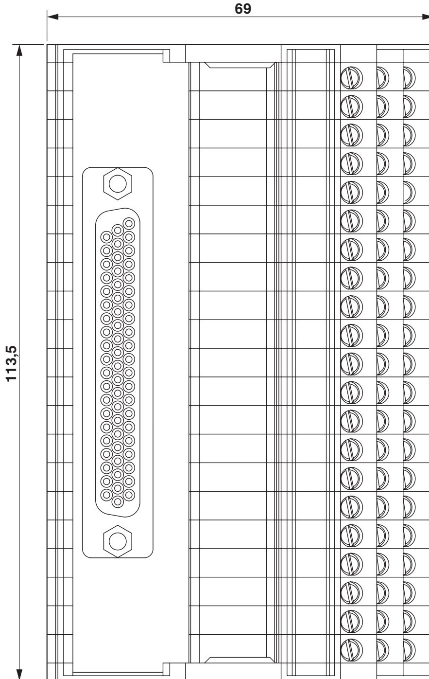
Dimensional drawing
