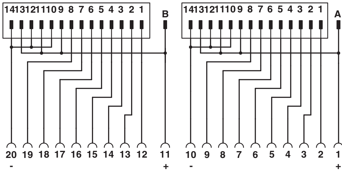
Circuit diagram
