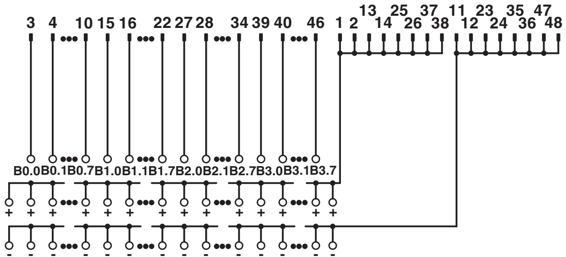
Connection scheme FLKMS 50/32IM/PLC
