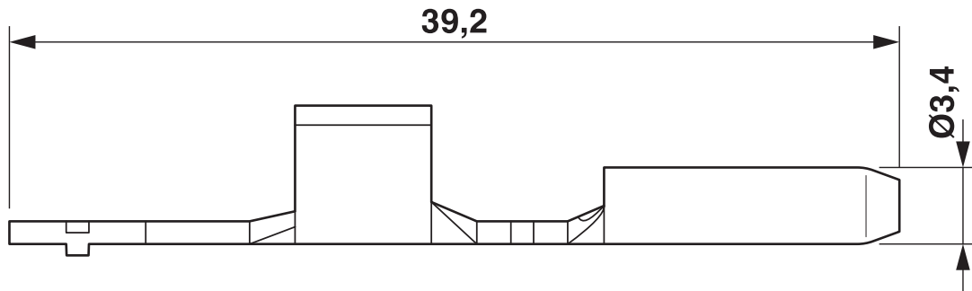
Dimensional drawing
