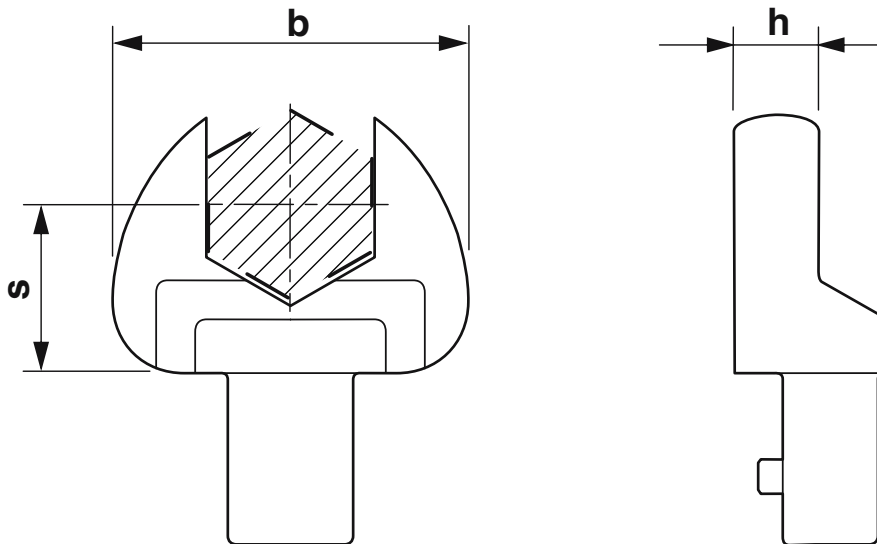
Dimensional drawing
