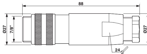
Dimensional drawing
