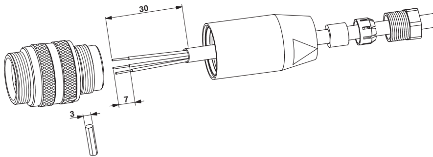
Functional drawing
