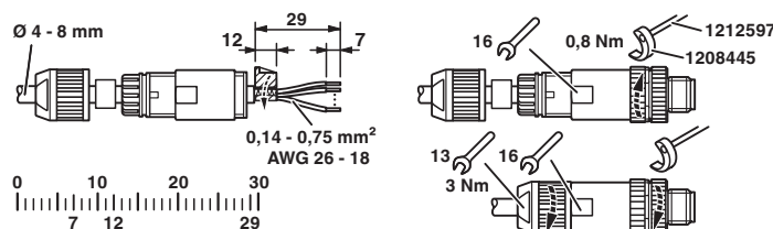
Functional drawing
