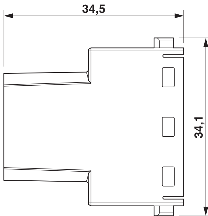
Dimensional drawing
