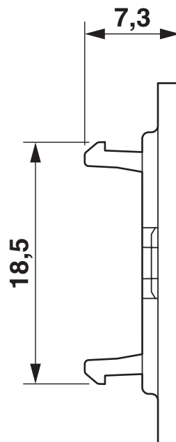
Dimensional drawing
