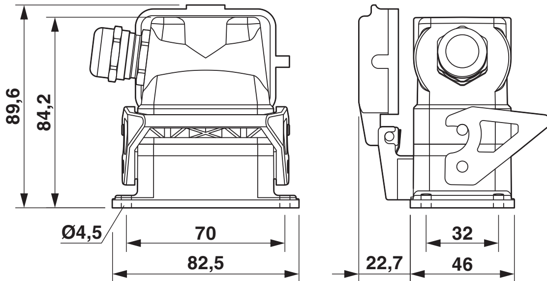
Dimensional drawing
