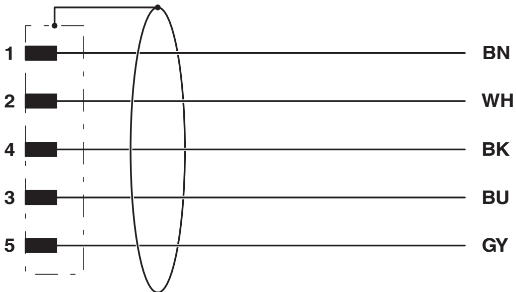
Contact assignment of the M12 plugs
