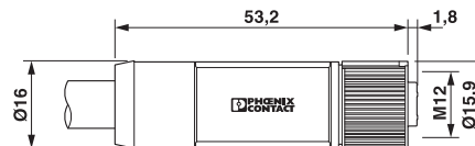
Dimensional drawing
