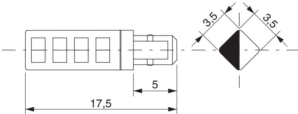
Dimensional drawing
