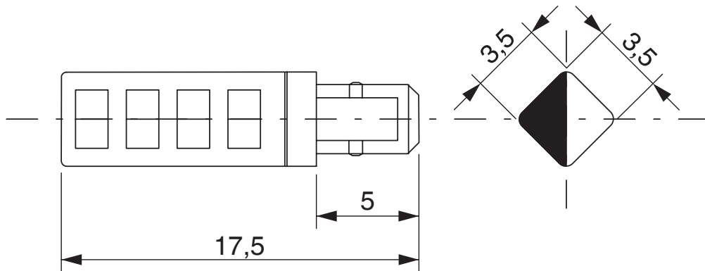
Dimensional drawing
