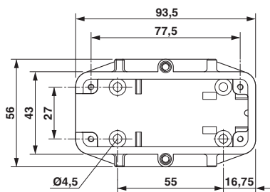
Dimensional drawing top view
