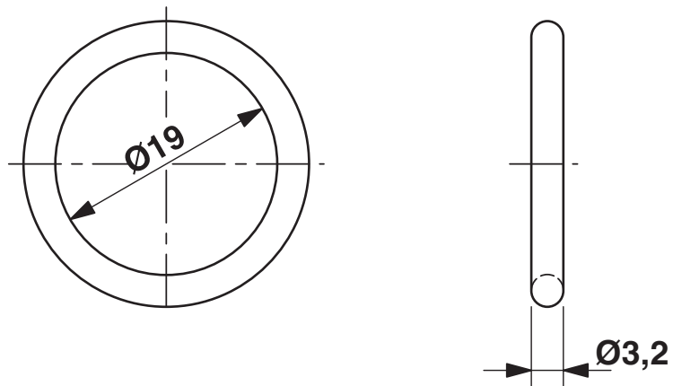
Dimensional drawing
