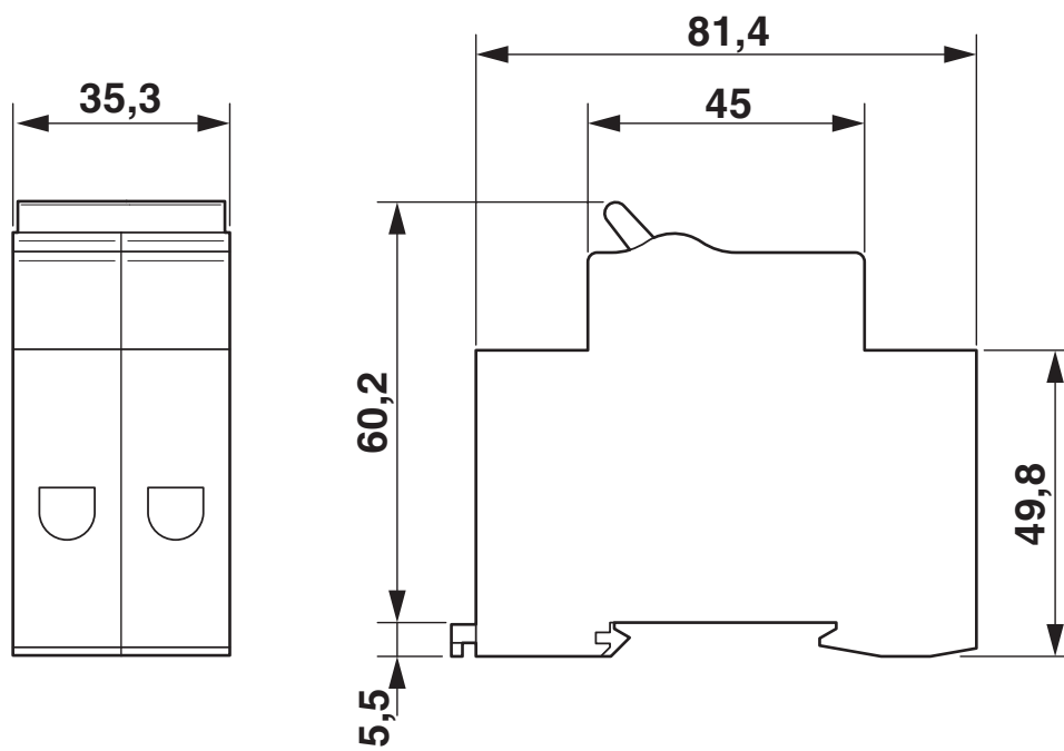
Dimensional drawing
