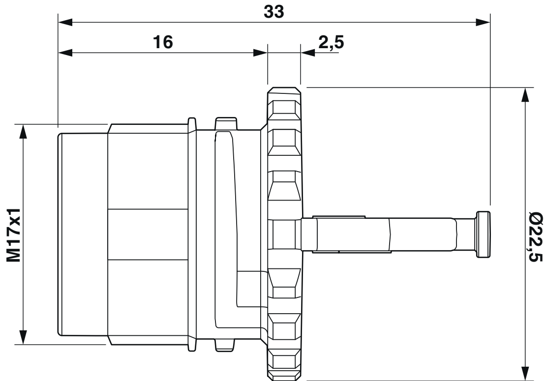
Dimensional drawing
