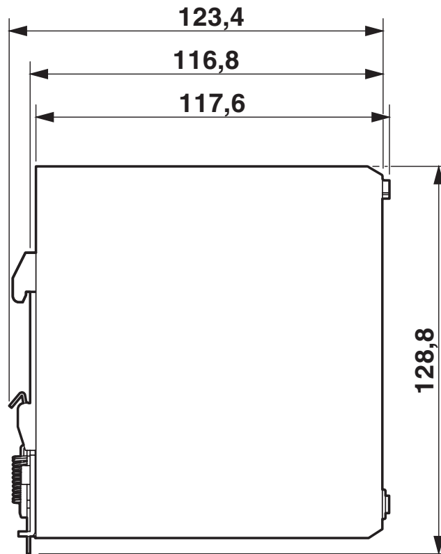
Dimensional drawing
