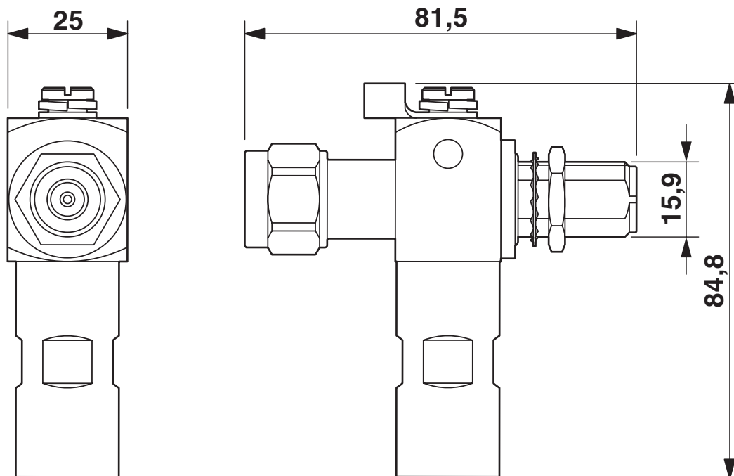
Dimensional drawing
