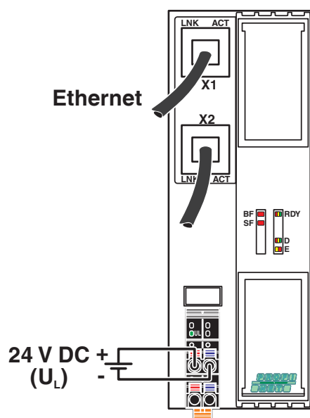
Connection diagram
