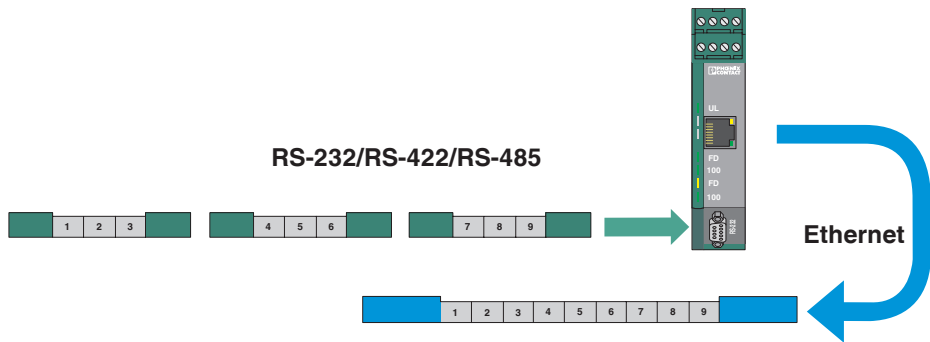
Application drawing
