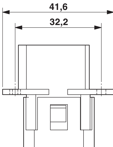
Dessin coté HC-COM-8-EBUC HC-COM-8-EBUC
