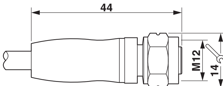
Dimensional drawing
