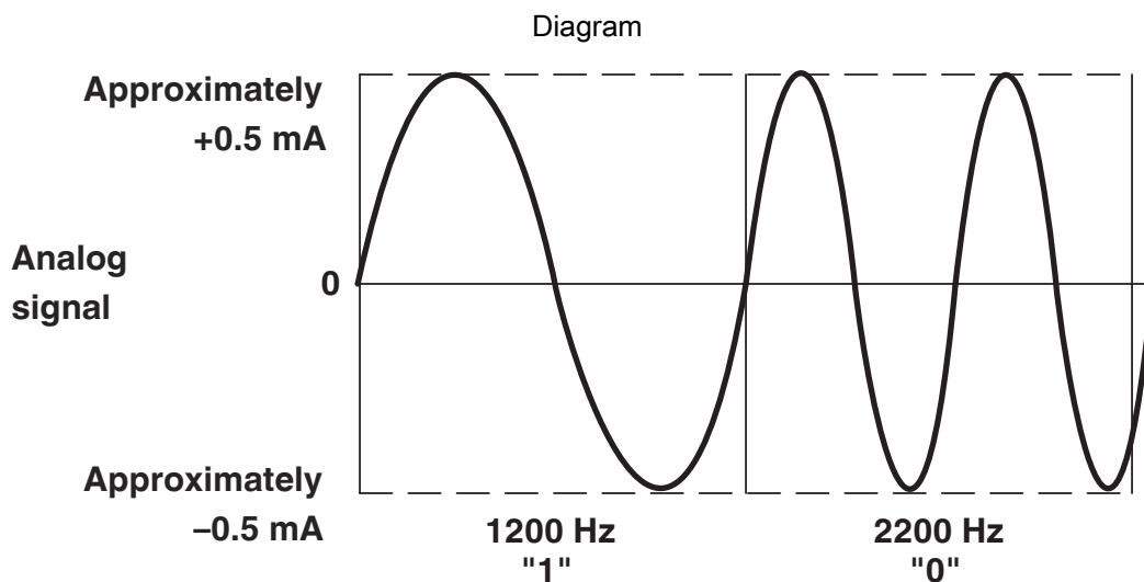
Signal transmission analog and digital at the same time
