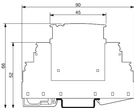
Figure 4. Dimensions
