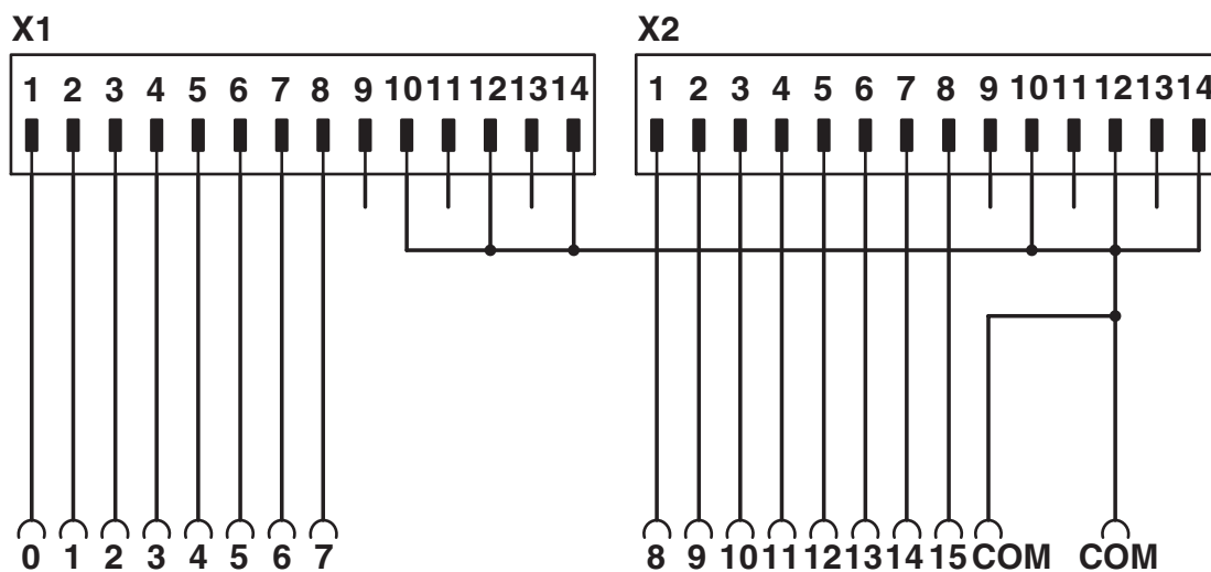
Kopplingsschema FLKM 14-PA-SLC500/IN
