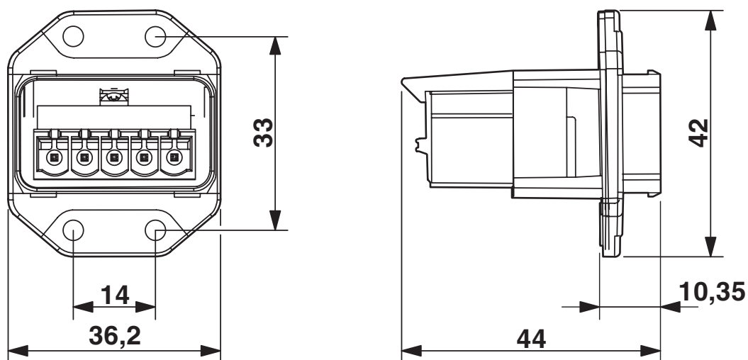
Push-Pull MSTB-montageram
