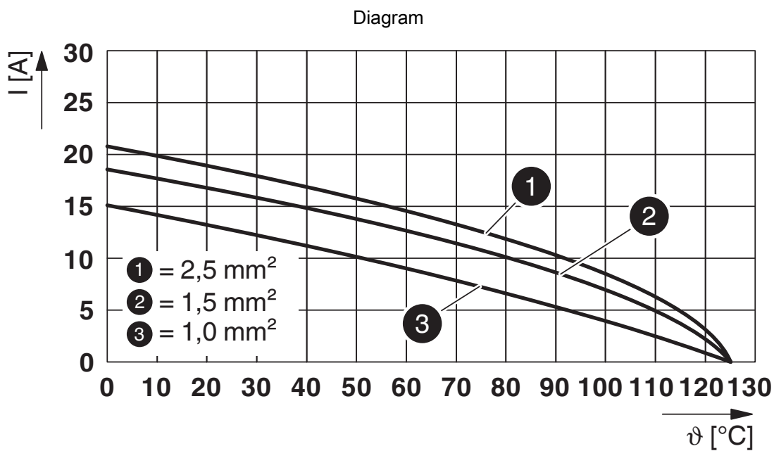
Derating-diagram rullade kontakter
