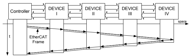
Figure 10. EtherCAT with 1 Gbps
