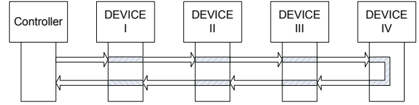
Figure 5. EtherCAT uses a ring structure
