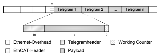
Figure 3. Structure of an EtherCAT-Frame
