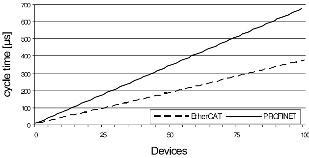
Figure 11. Cycle time as a function of the number of devices with a constant payload of 16 byte per device and a bit rate of 100Mbps
