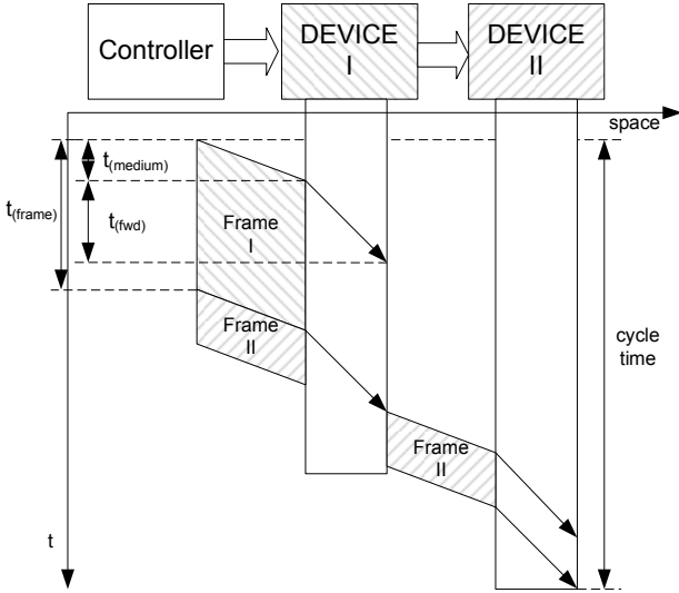
Figure 6. Space-time Diagram
