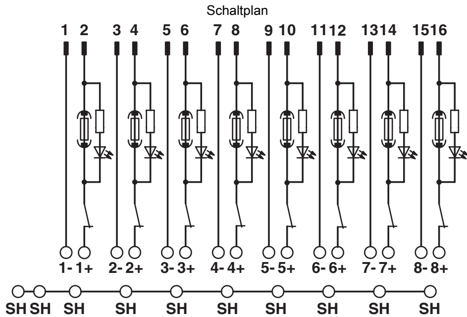
Anschlussbild VIP-PT/FLK16/DS/FU/LED/AN/DV
