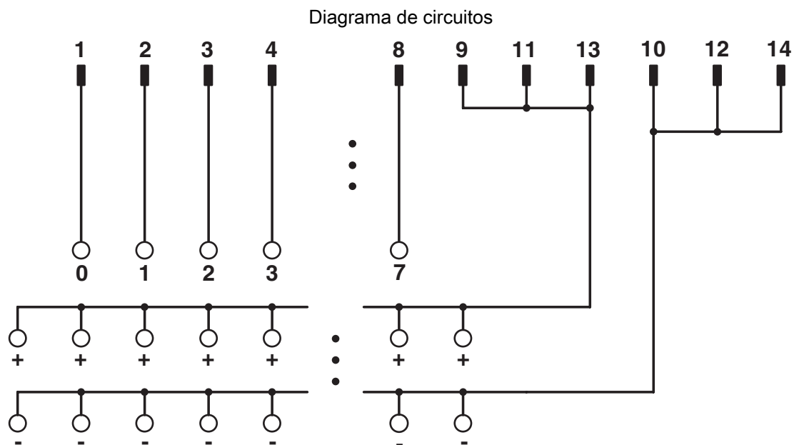
Diagrama de conexões FLKMS 14/8IM/PLC
